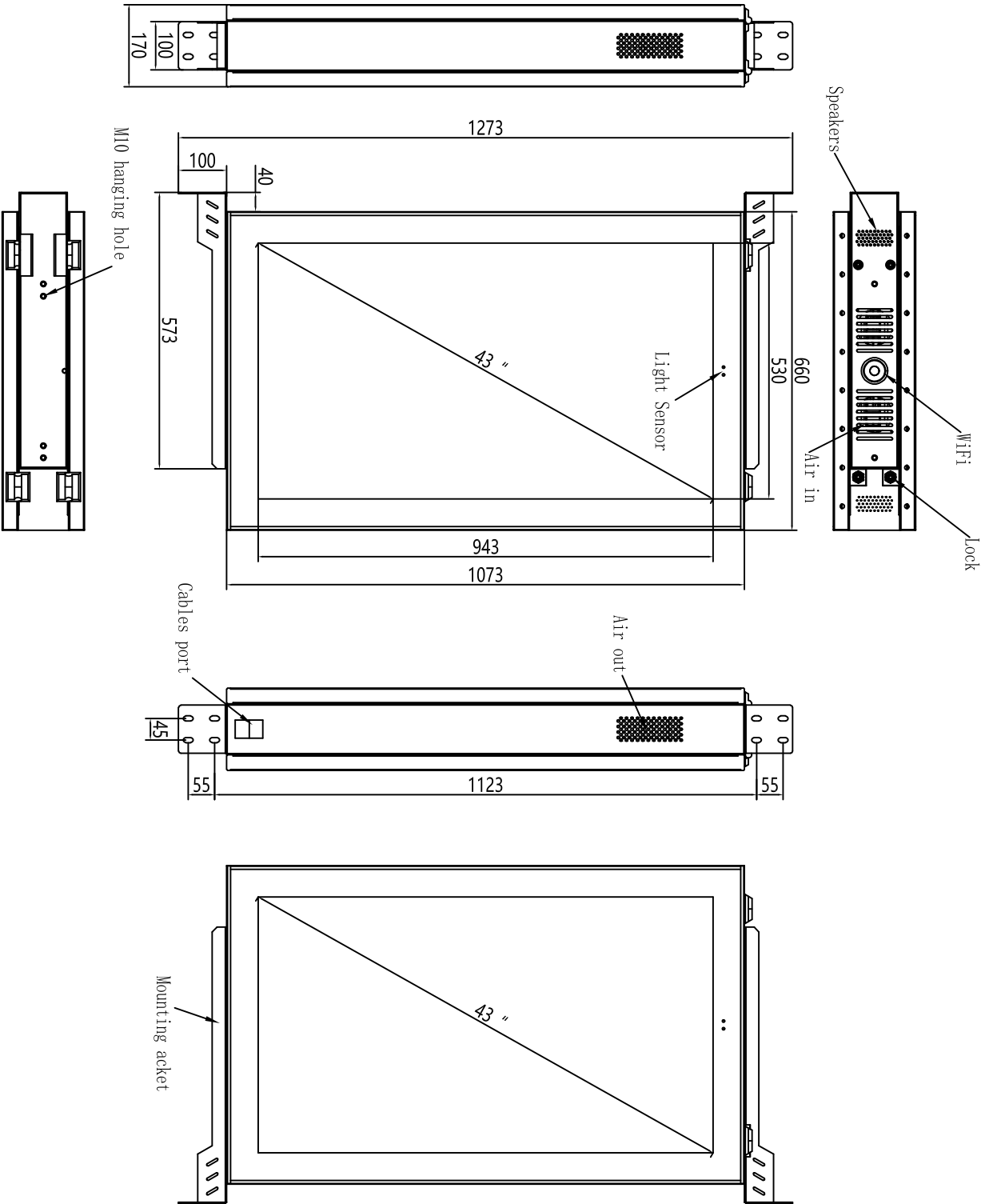
43inch dual side pole LCD digital signage
